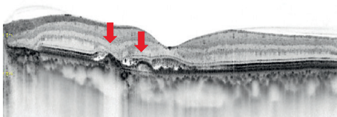
OCT image
