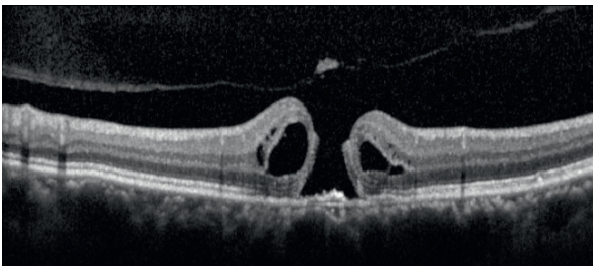
Preoperative OCT
