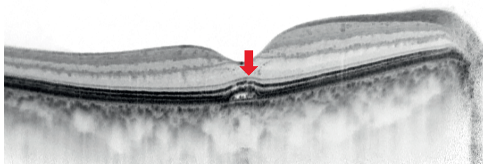
OCT image
